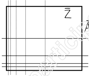
Figure 3: z -solutions are convergent power series in z with coefficients in \mathbb{Q}(a) , and the poles (solid lines in the picture) of these coefficients accumulate to a = 0_{\mathfrak{e}} . The poles of a -solutions, the dashed lines in the figure, similarly accumulate to z = 0_X .
